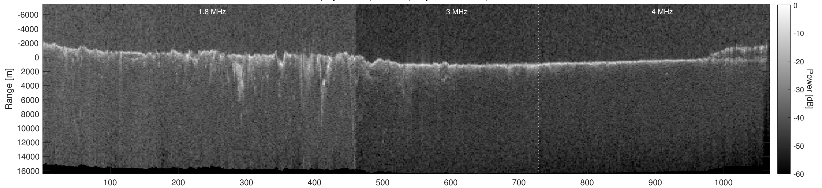
Orbit 5931, Depth-Corrected Cluttergram
