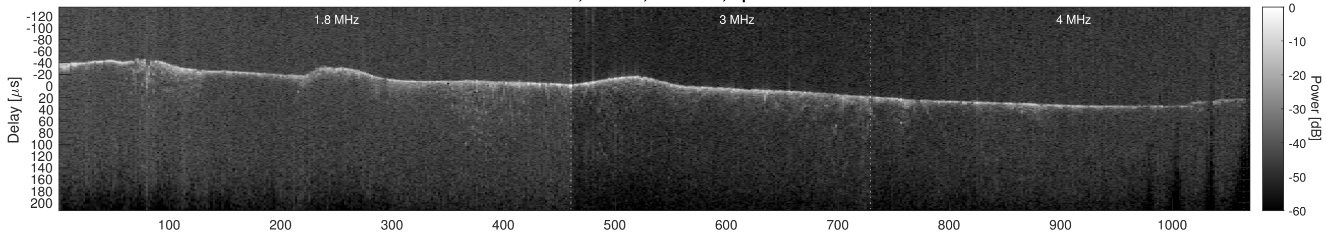
Orbit 5932, Cluttergram
