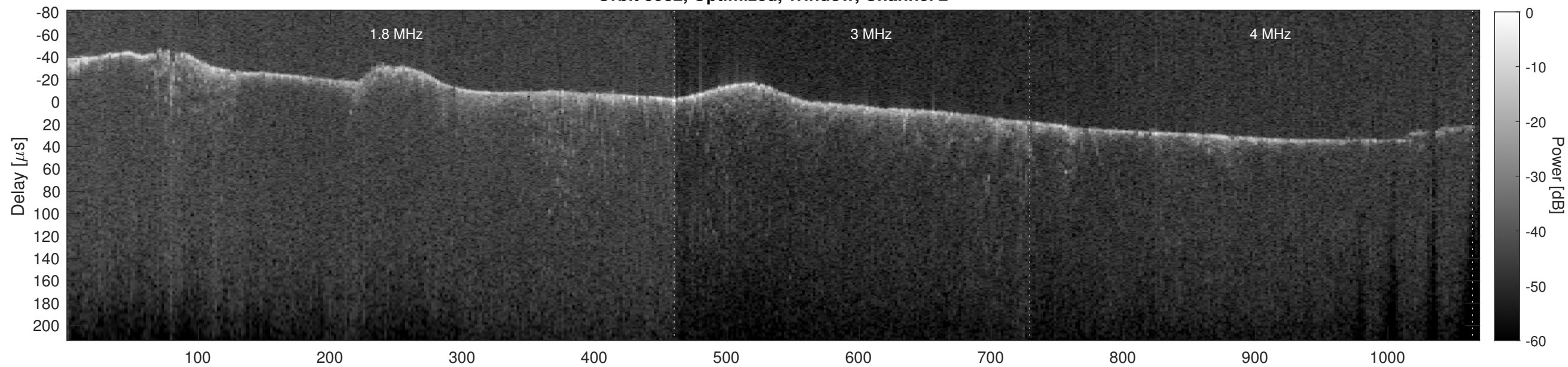
Orbit 5932, Cluttergram
