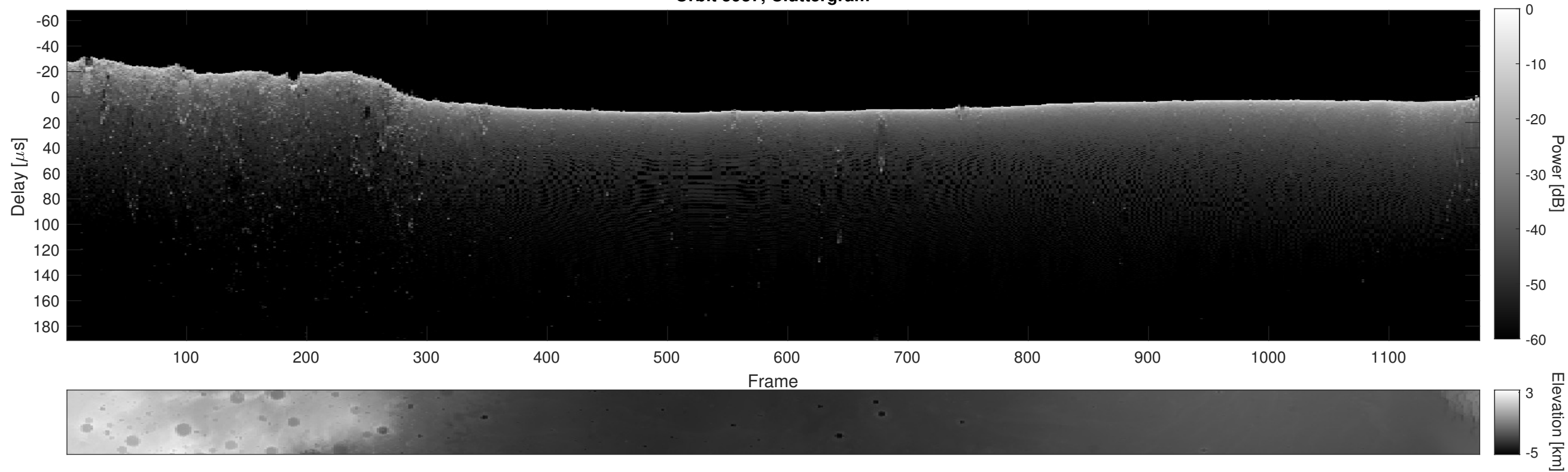
Orbit 5937, Cluttergram
