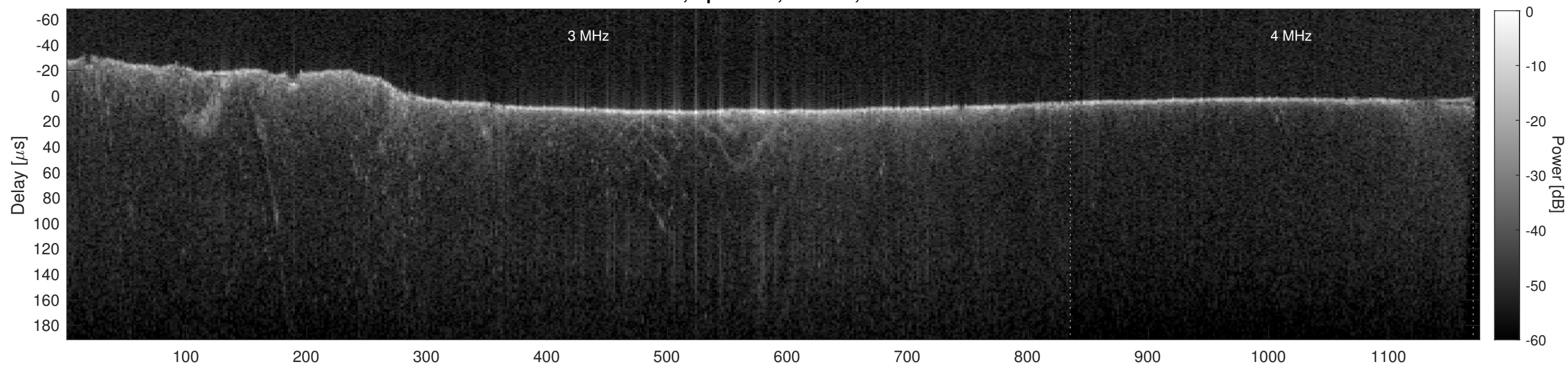
Orbit 5937, Cluttergram
