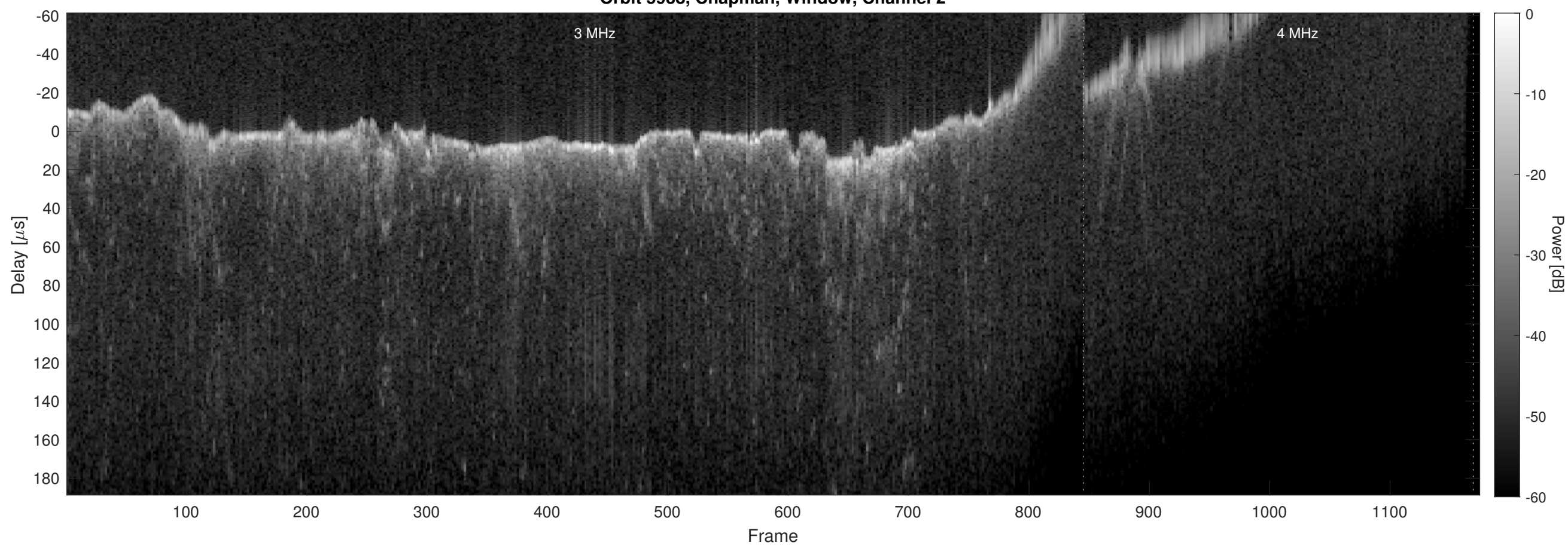
Orbit 5938, Chapman, Window, Channel 2
