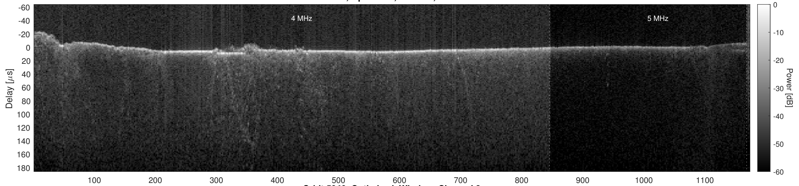
Orbit 5940, Optimized, Window, Channel 2
