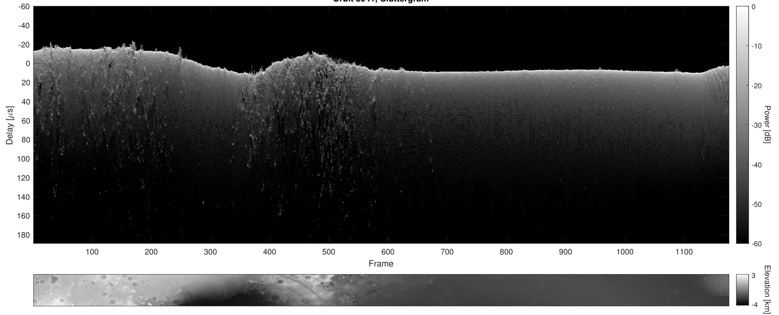
Orbit 5941, Cluttergram
