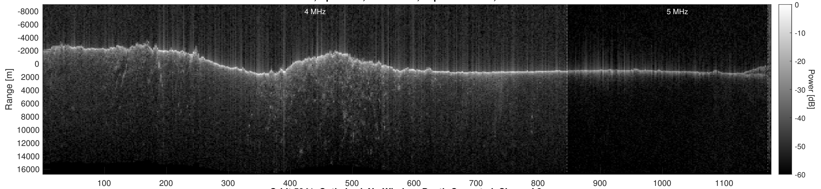
Orbit 5941, Optimized, No Window, Depth-Corrected, Channel 2
