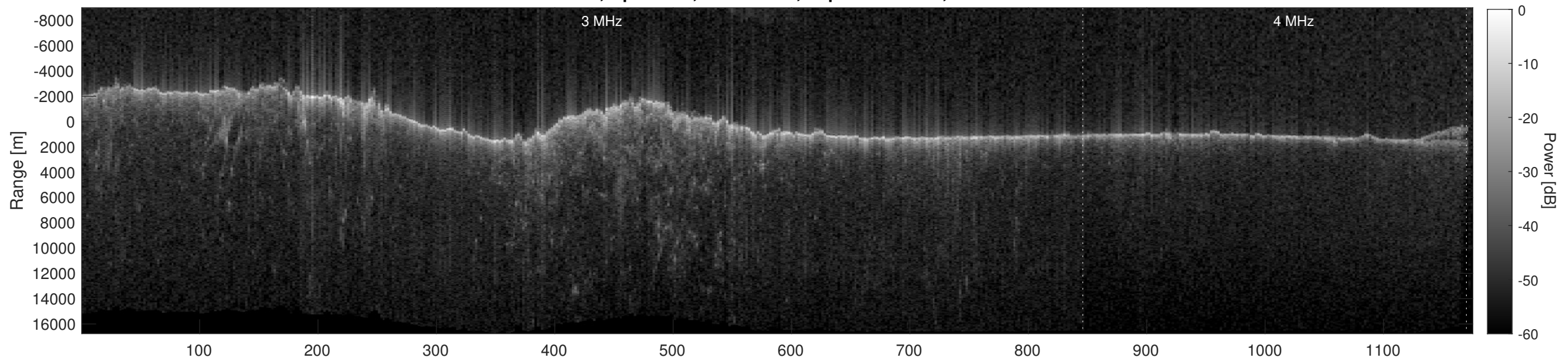
Orbit 5941, Depth-Corrected Cluttergram
