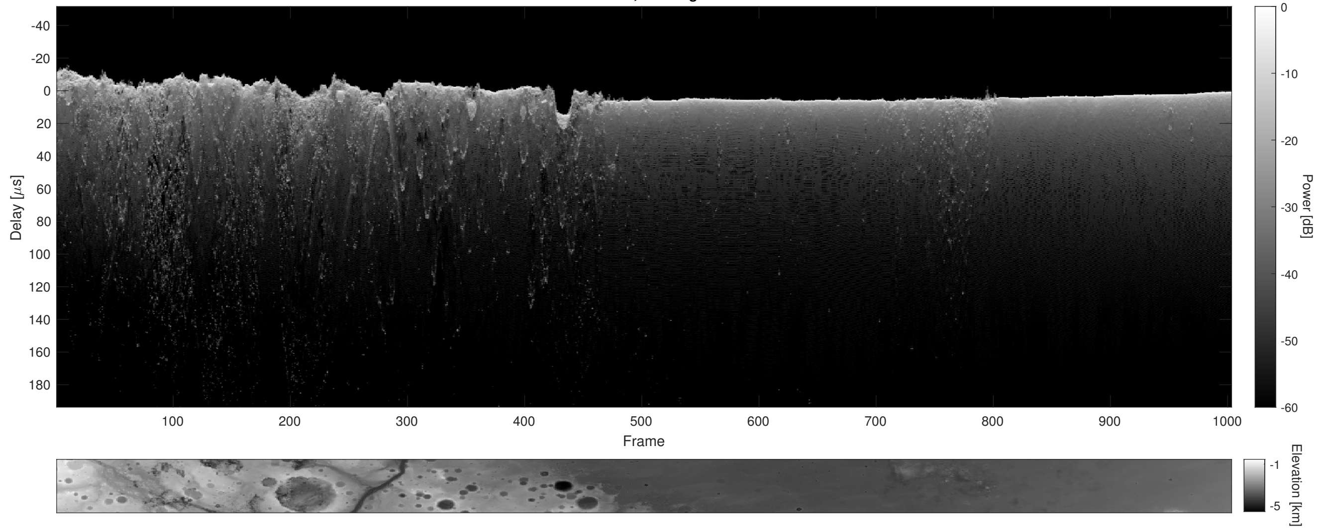
Orbit 5942, Cluttergram
