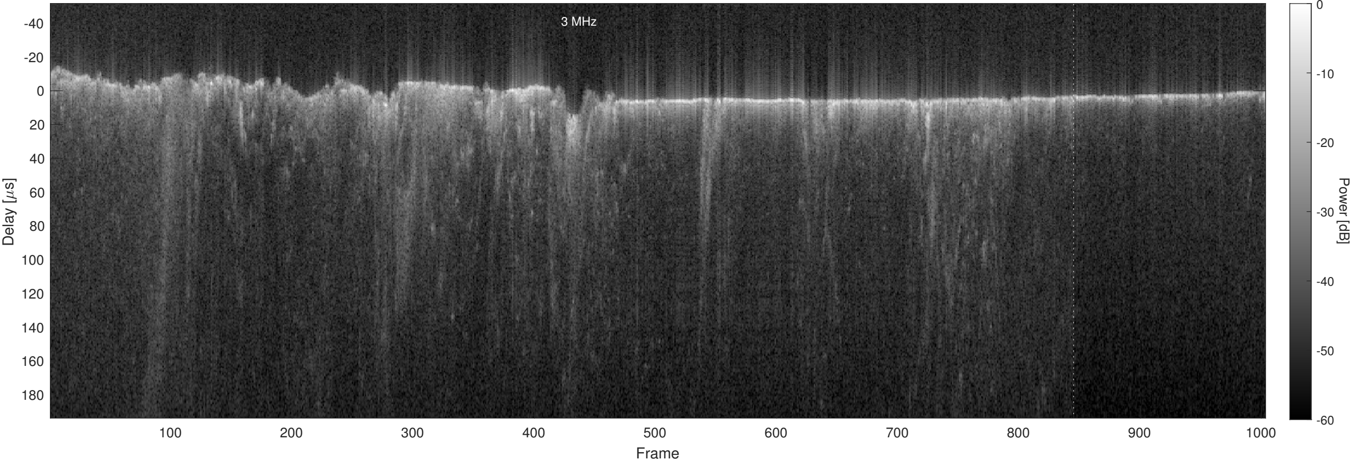
Orbit 5942, Optimized, No Window, Channel 2
