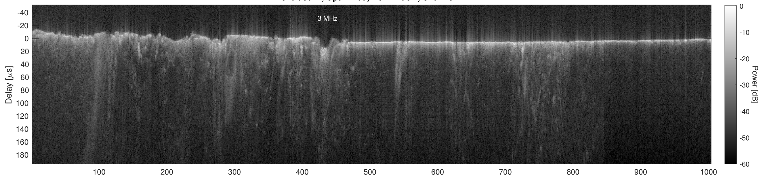
Orbit 5942, Cluttergram
