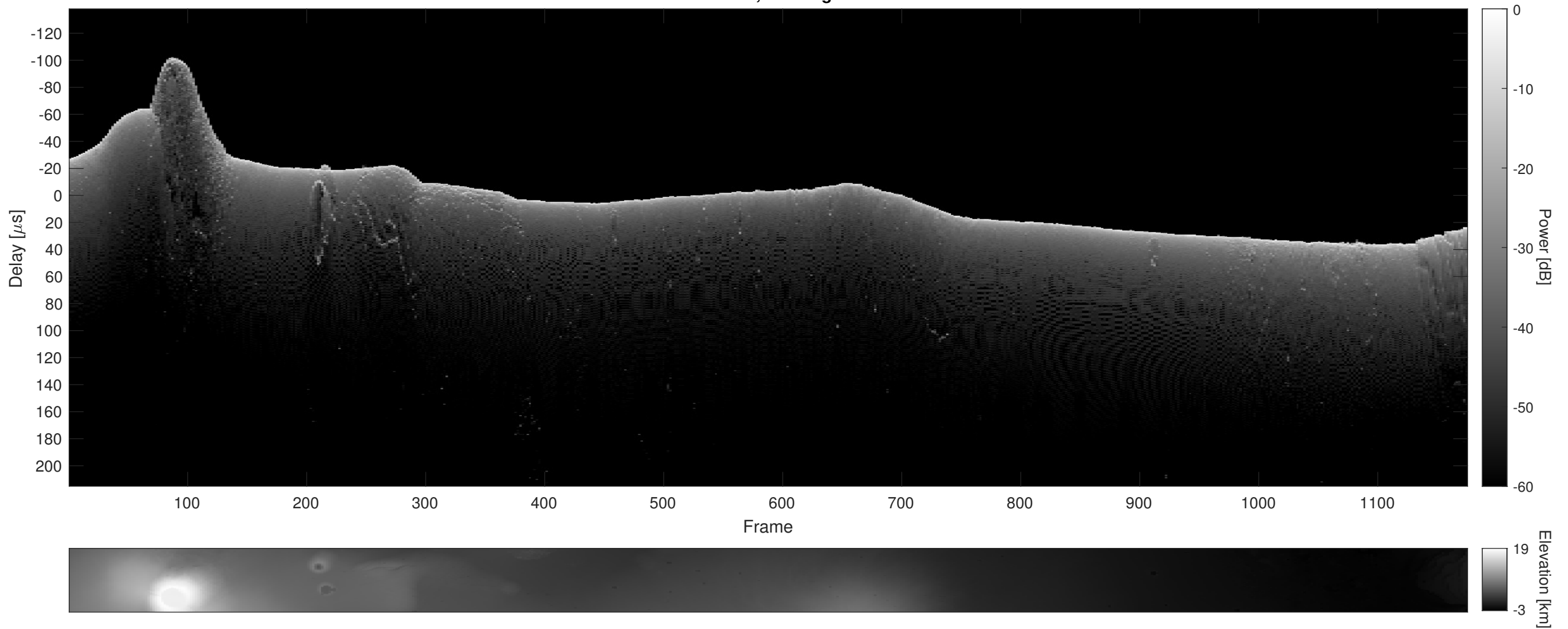
Orbit 5943, Cluttergram
