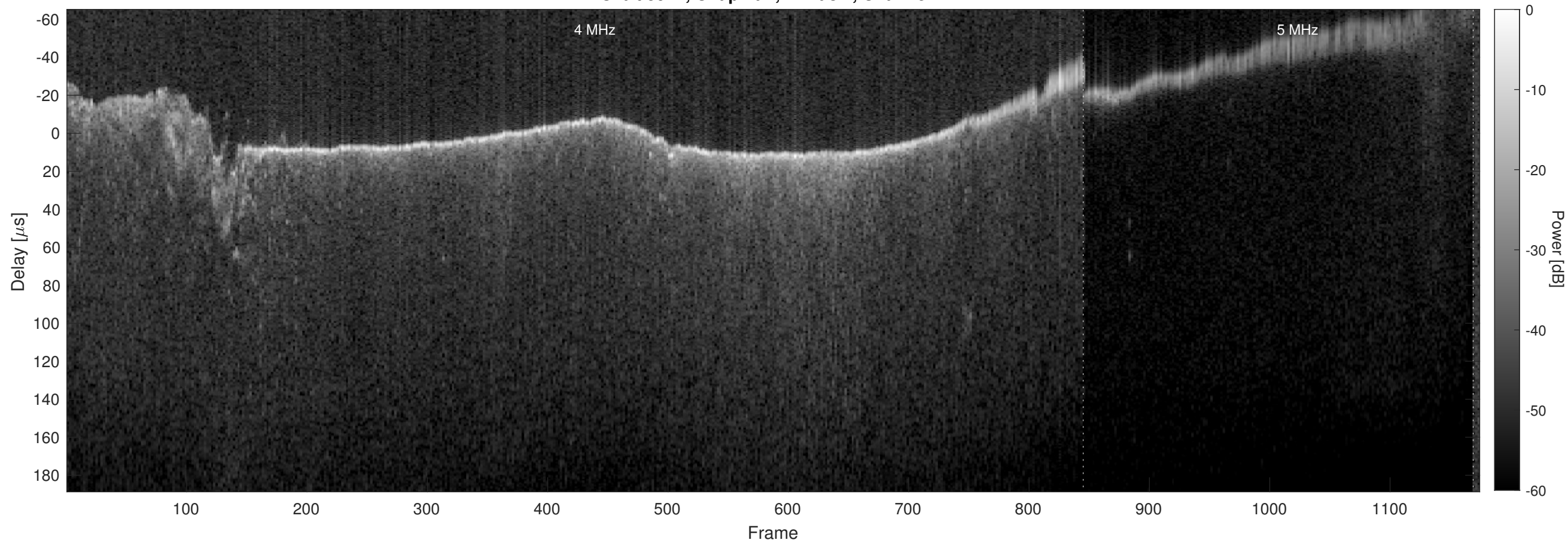
Orbit 5944, Chapman, Window, Channel 2
