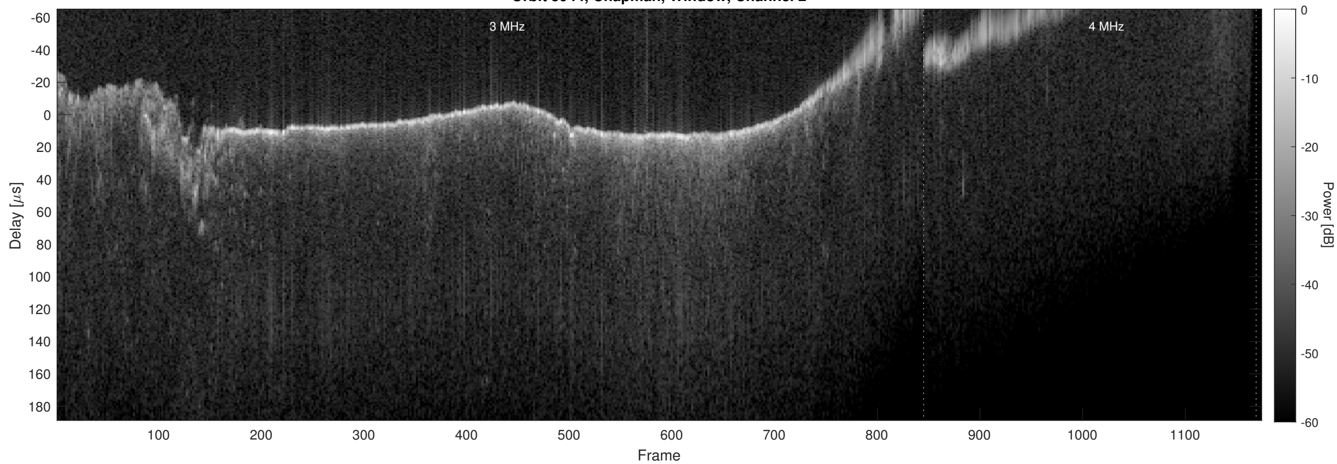
Orbit 5944, Chapman, Window, Channel 2
