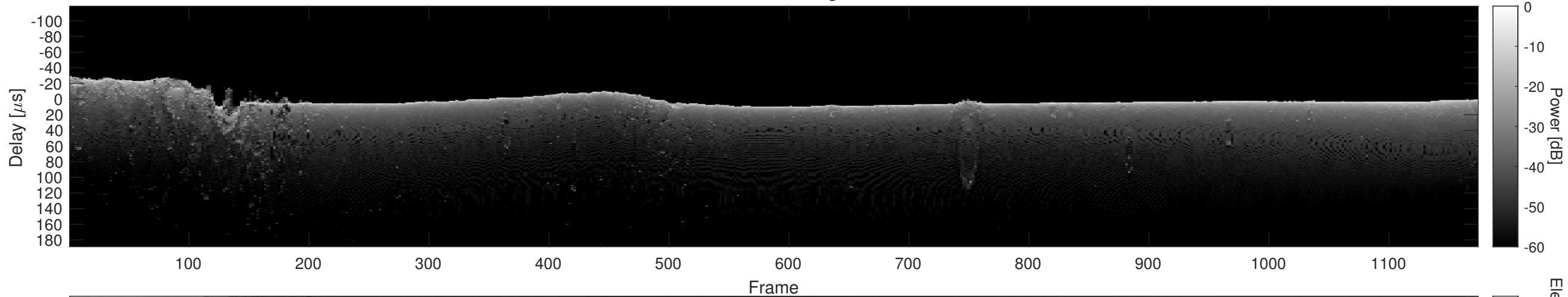
Orbit 5944, Cluttergram
