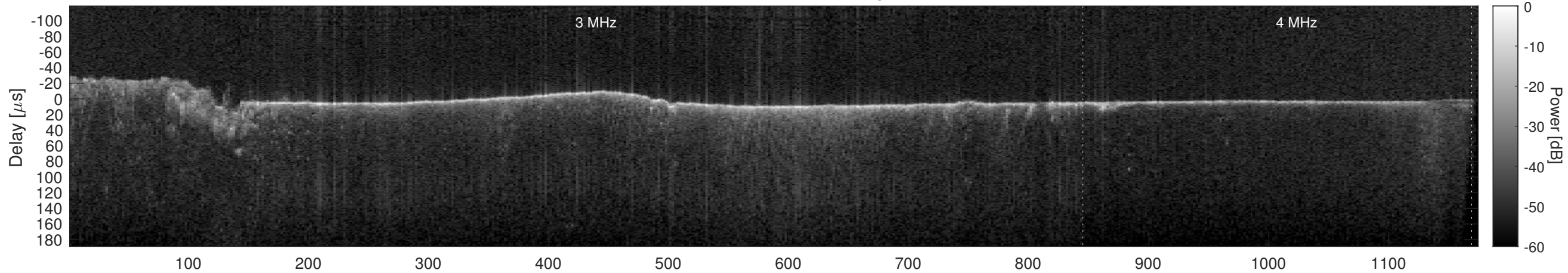
Orbit 5944, Cluttergram
