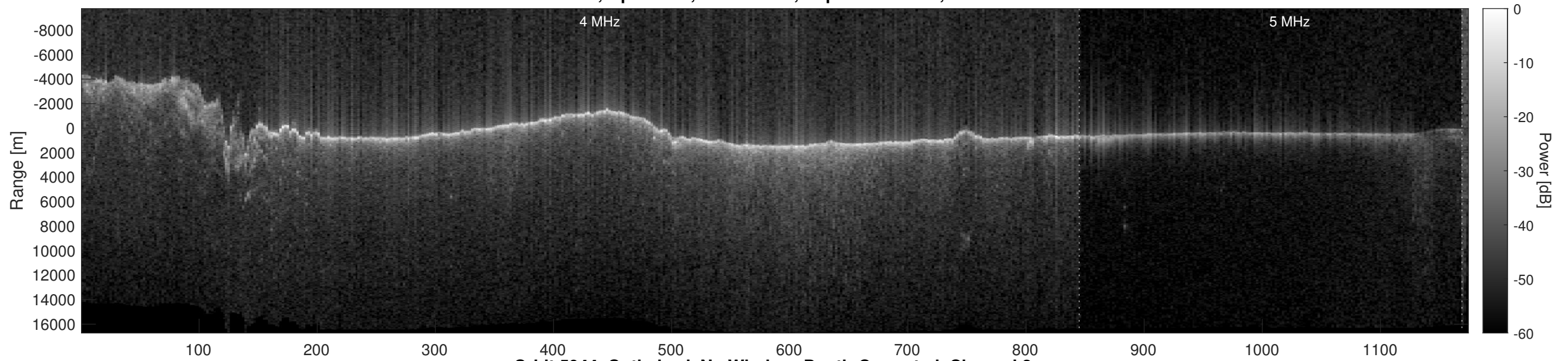
Orbit 5944, Optimized, No Window, Depth-Corrected, Channel 2
