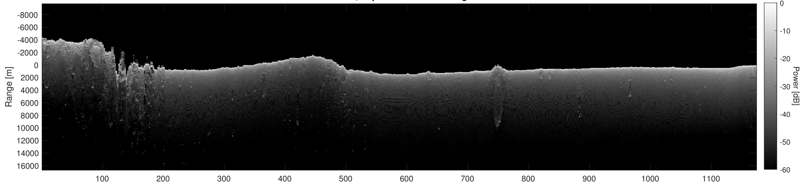
Orbit 5944, Depth-Corrected Cluttergram
