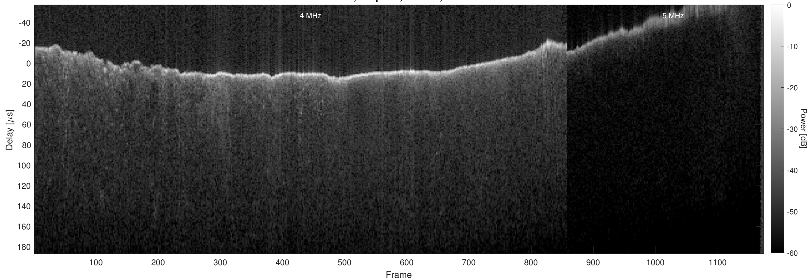
Orbit 5947, Chapman, Window, Channel 2
