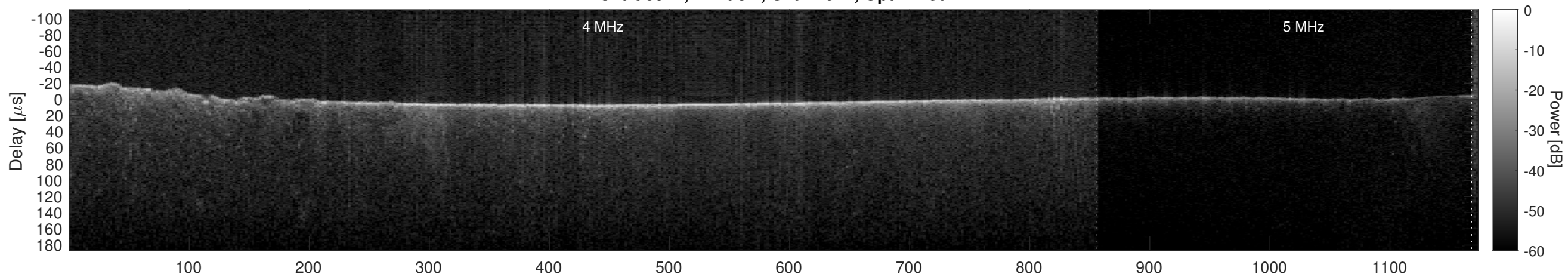
Orbit 5947, Cluttergram
