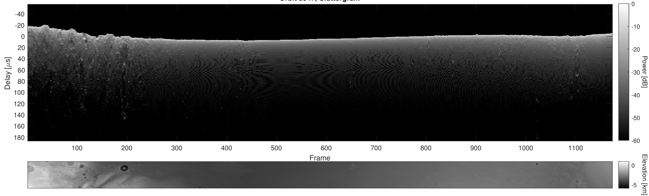
Orbit 5947, Cluttergram
