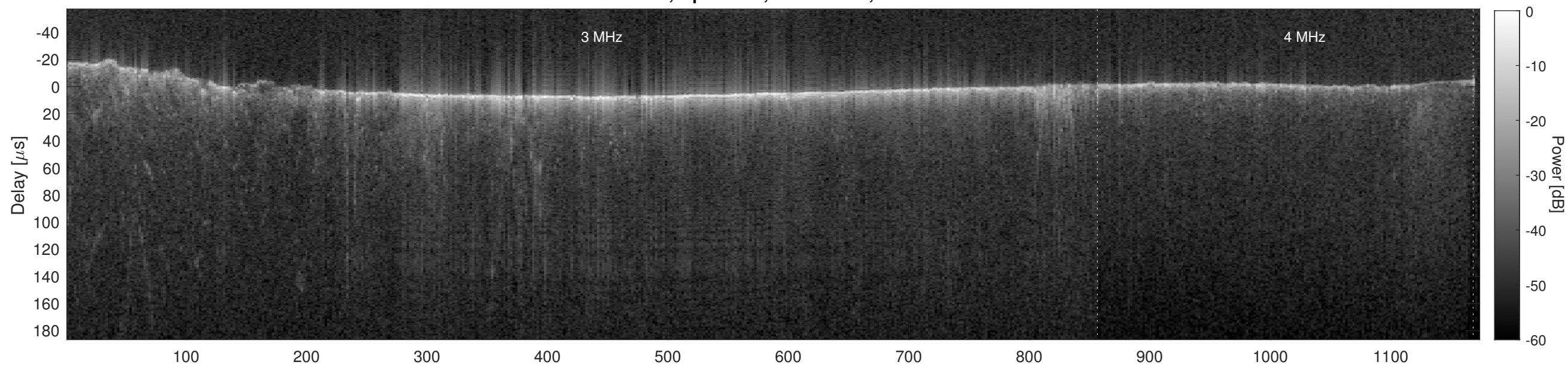
Orbit 5947, Cluttergram
