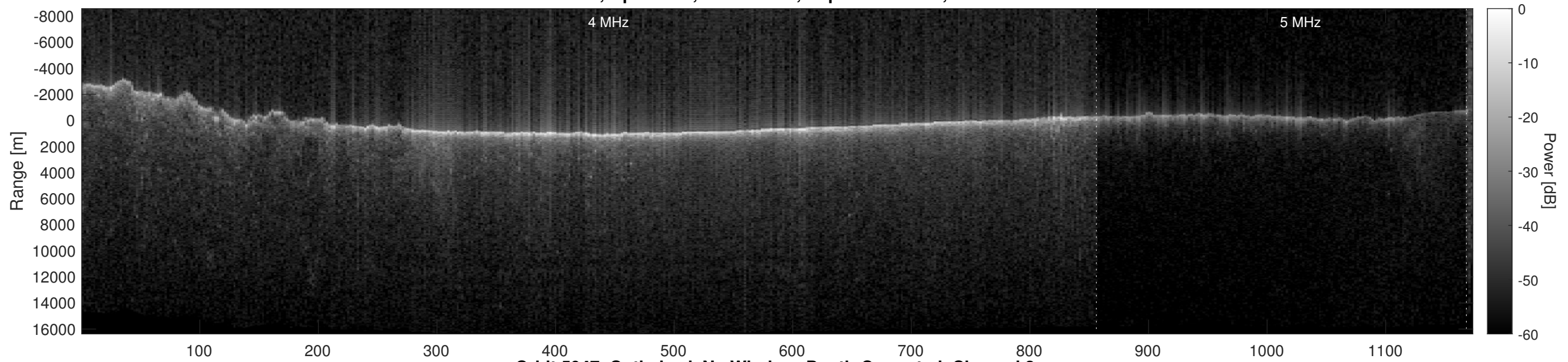
Orbit 5947, Optimized, No Window, Depth-Corrected, Channel 2
