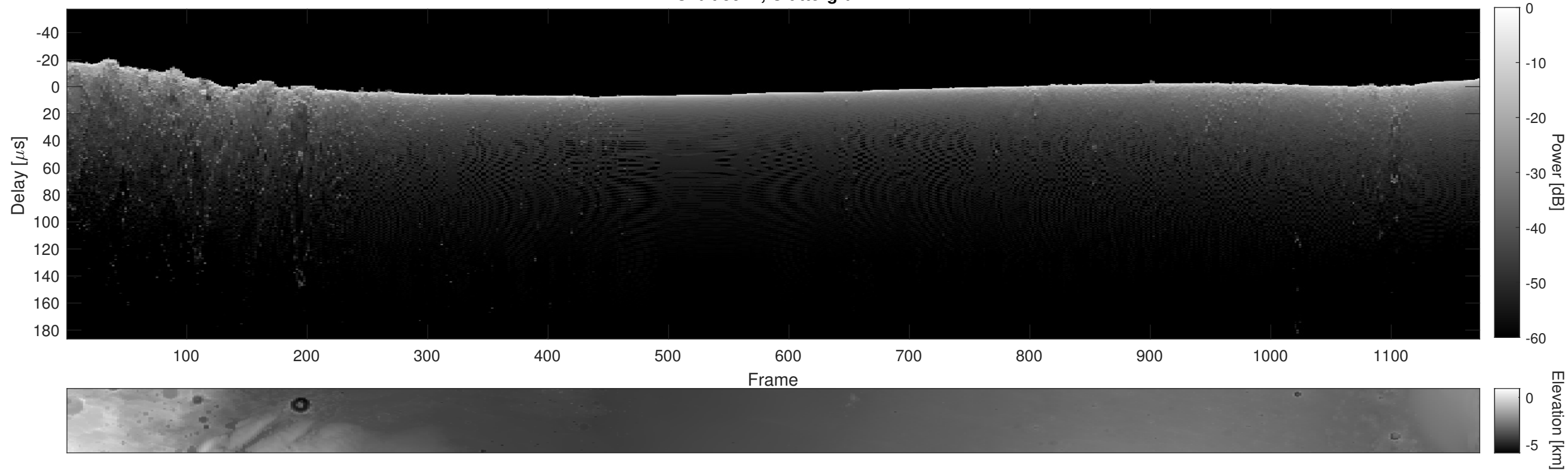
Orbit 5947, Cluttergram
