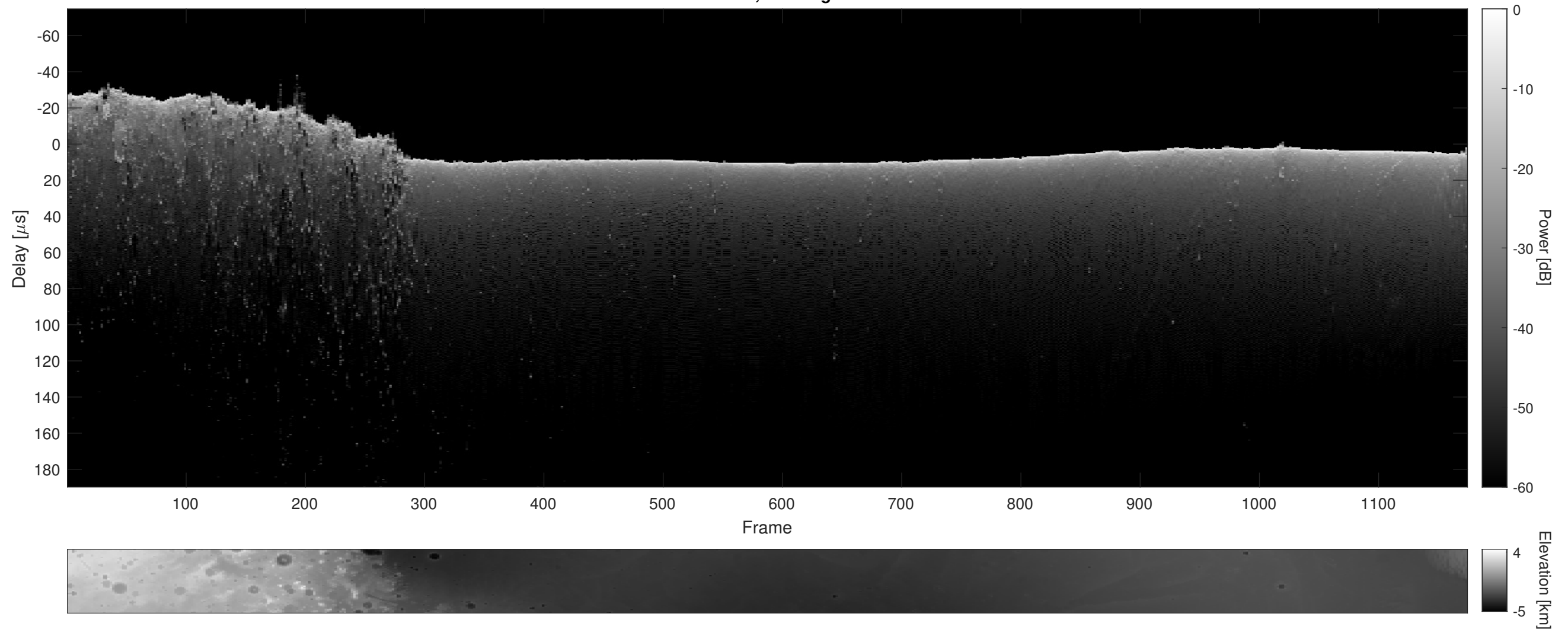
Orbit 5948, Cluttergram
