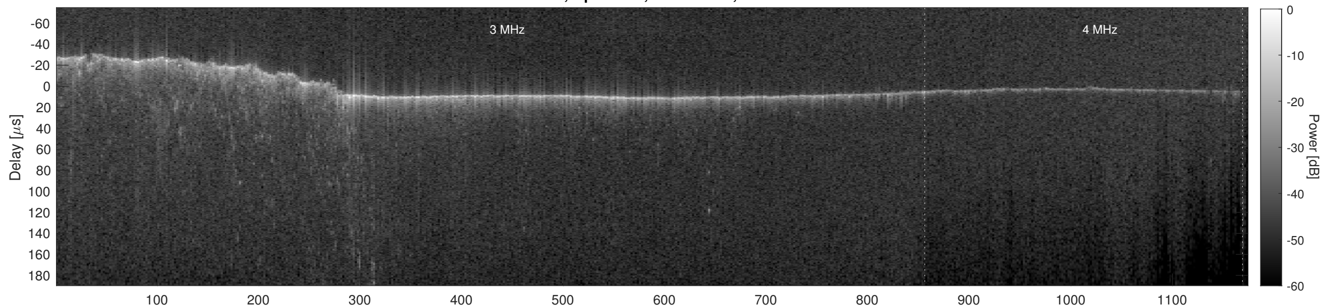
Orbit 5948, Cluttergram
