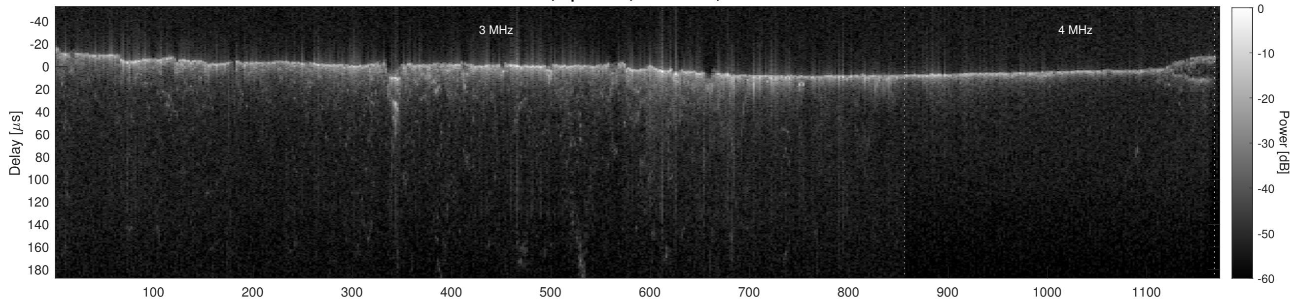
Orbit 5949, Cluttergram
