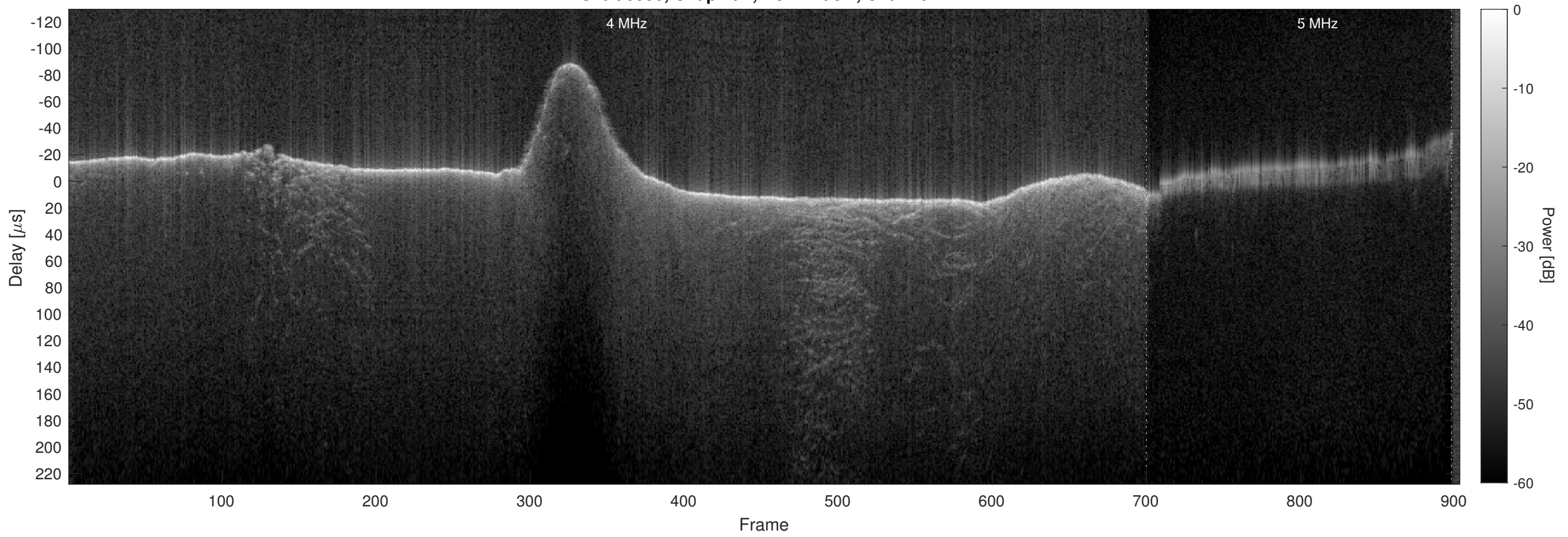
Orbit 5950, Chapman, No Window, Channel 2
