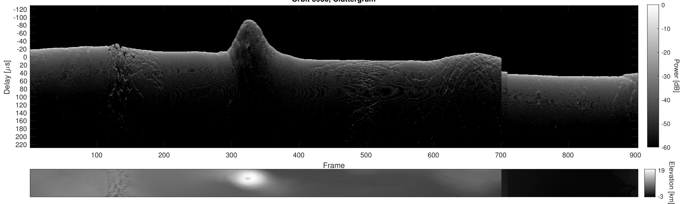
Orbit 5950, Cluttergram
