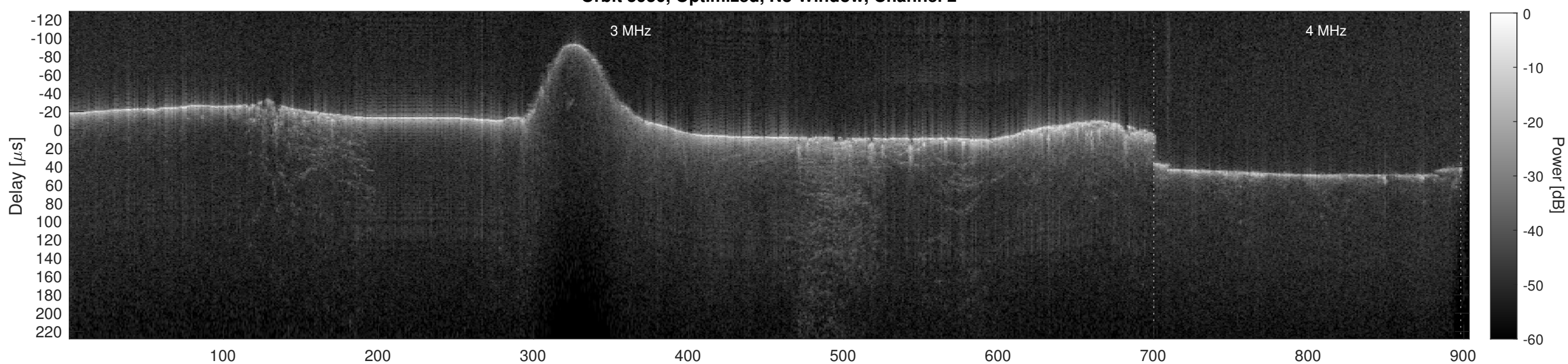
Orbit 5950, Cluttergram
