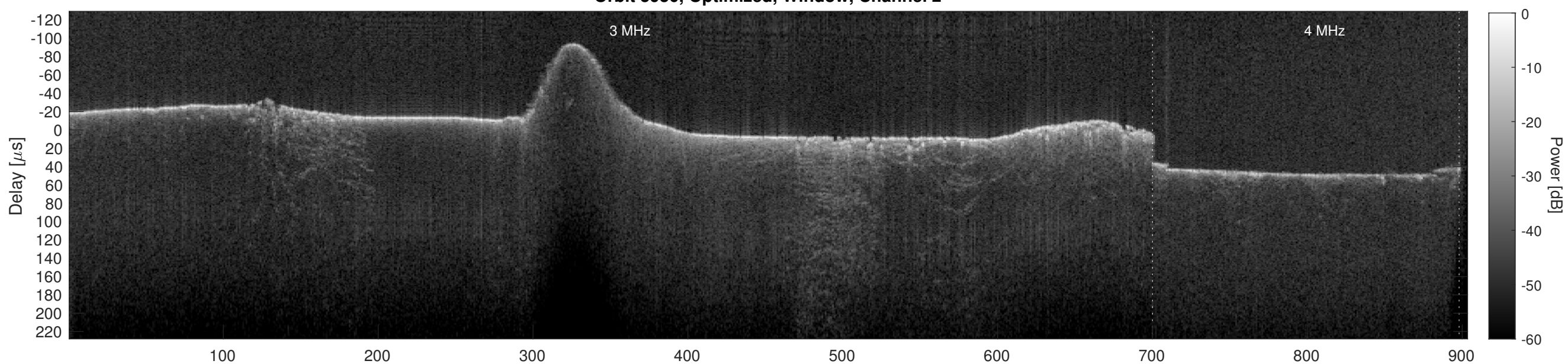
Orbit 5950, Cluttergram
