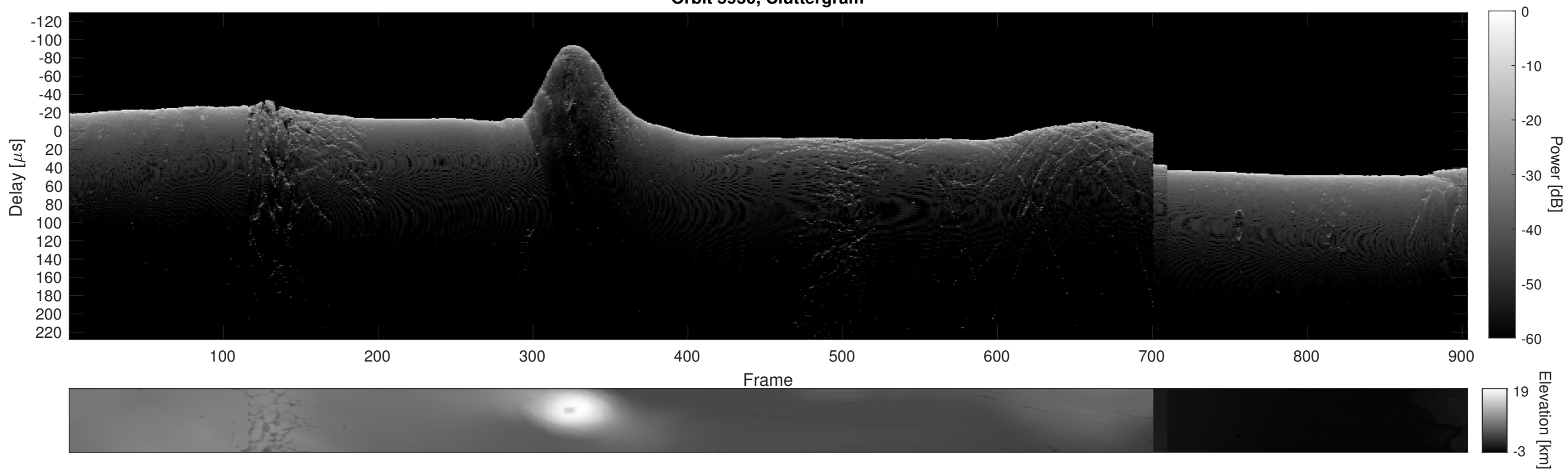
Orbit 5950, Cluttergram
