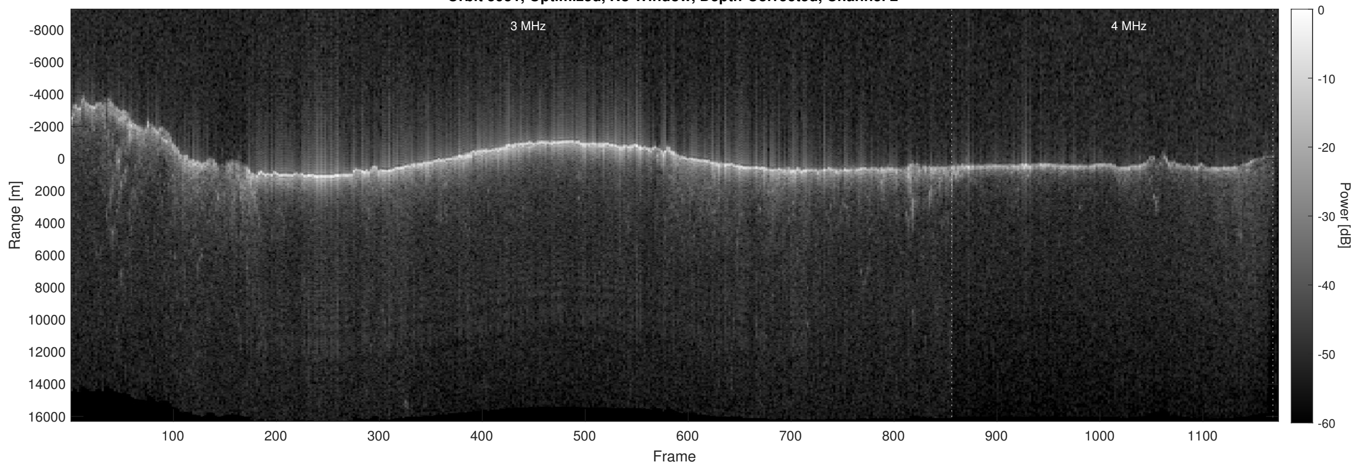
Orbit 5951, Optimized, No Window, Depth-Corrected, Channel 2
