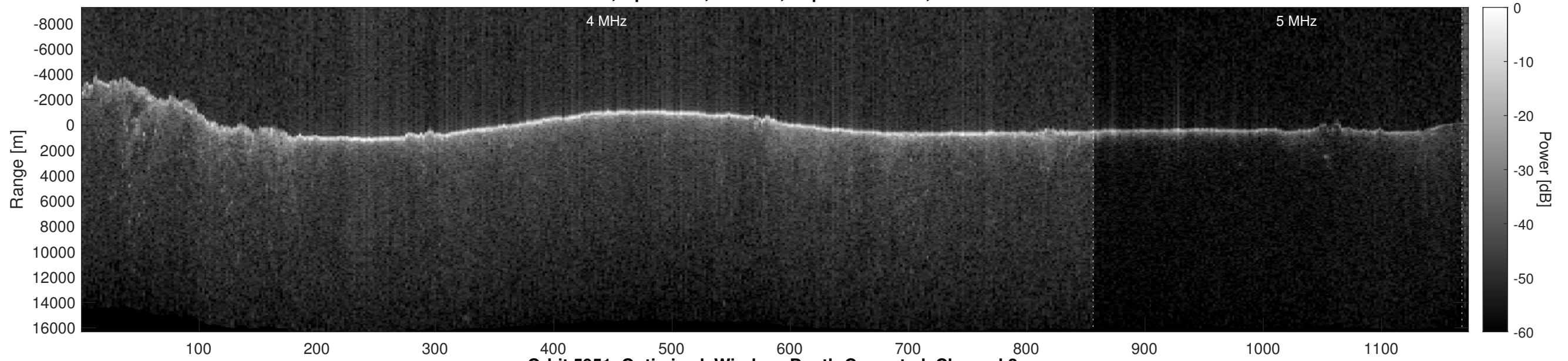
Orbit 5951, Optimized, Window, Depth-Corrected, Channel 2
