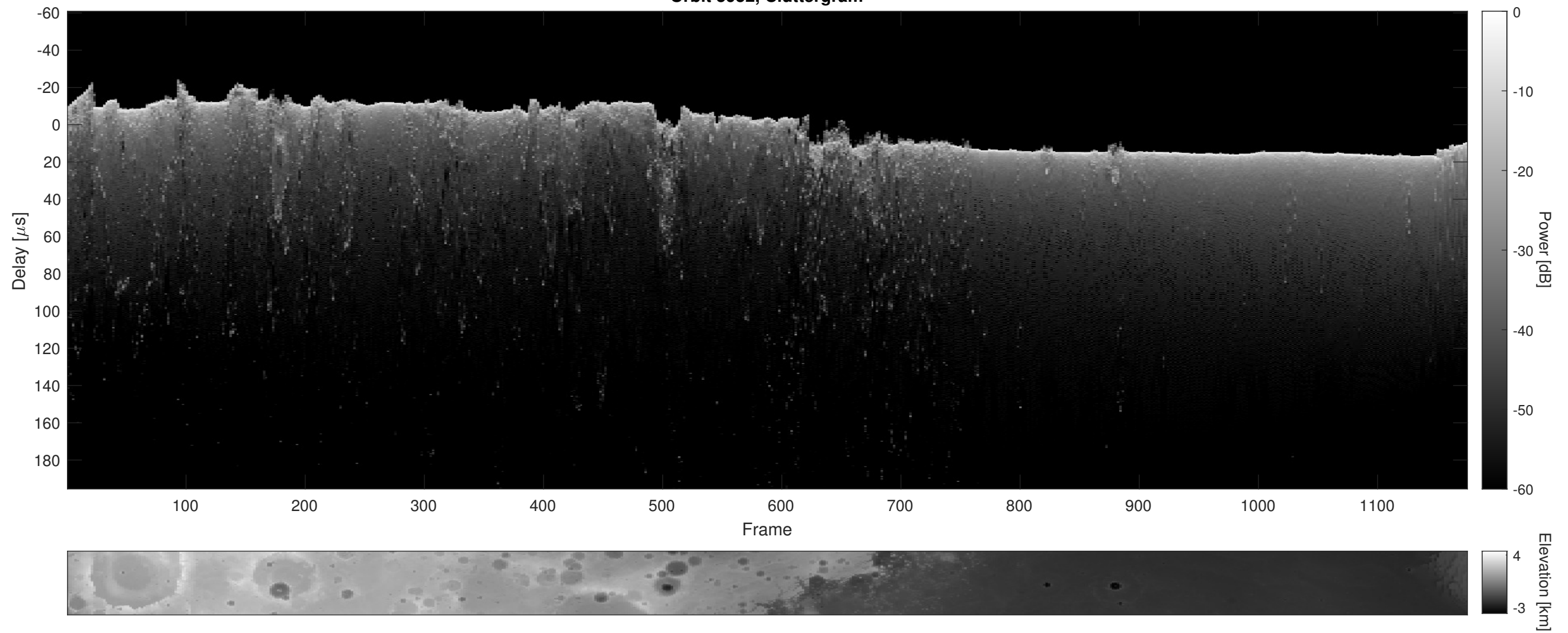
Orbit 5952, Cluttergram
