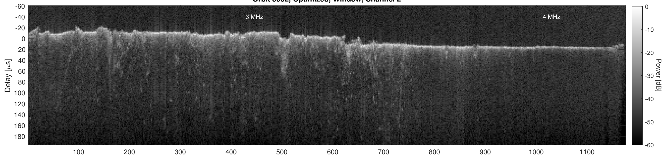
Orbit 5952, Cluttergram
