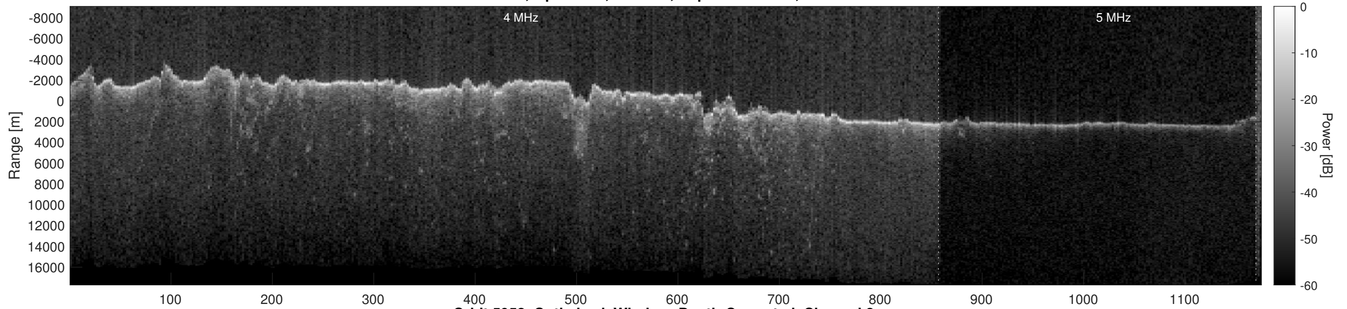
Orbit 5952, Optimized, Window, Depth-Corrected, Channel 2
