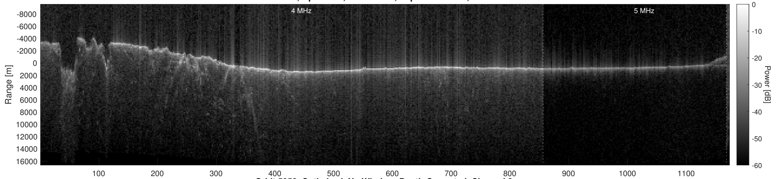
Orbit 5953, Optimized, No Window, Depth-Corrected, Channel 2
