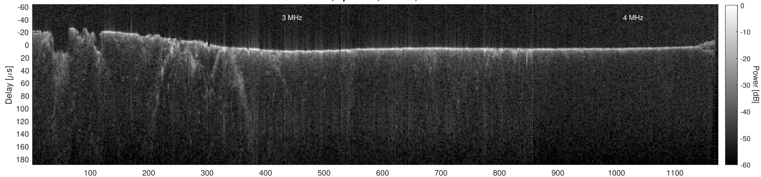
Orbit 5953, Cluttergram
