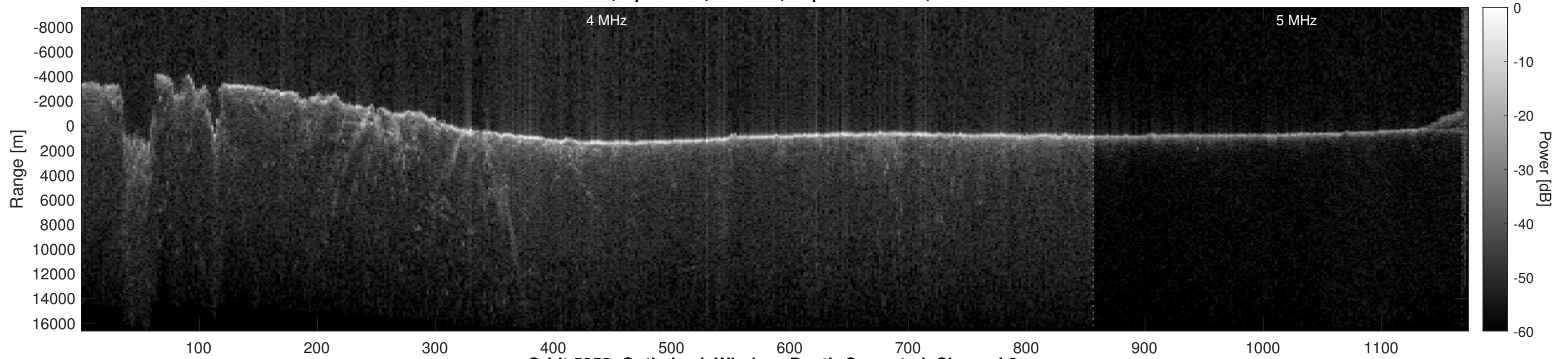
Orbit 5953, Optimized, Window, Depth-Corrected, Channel 2
