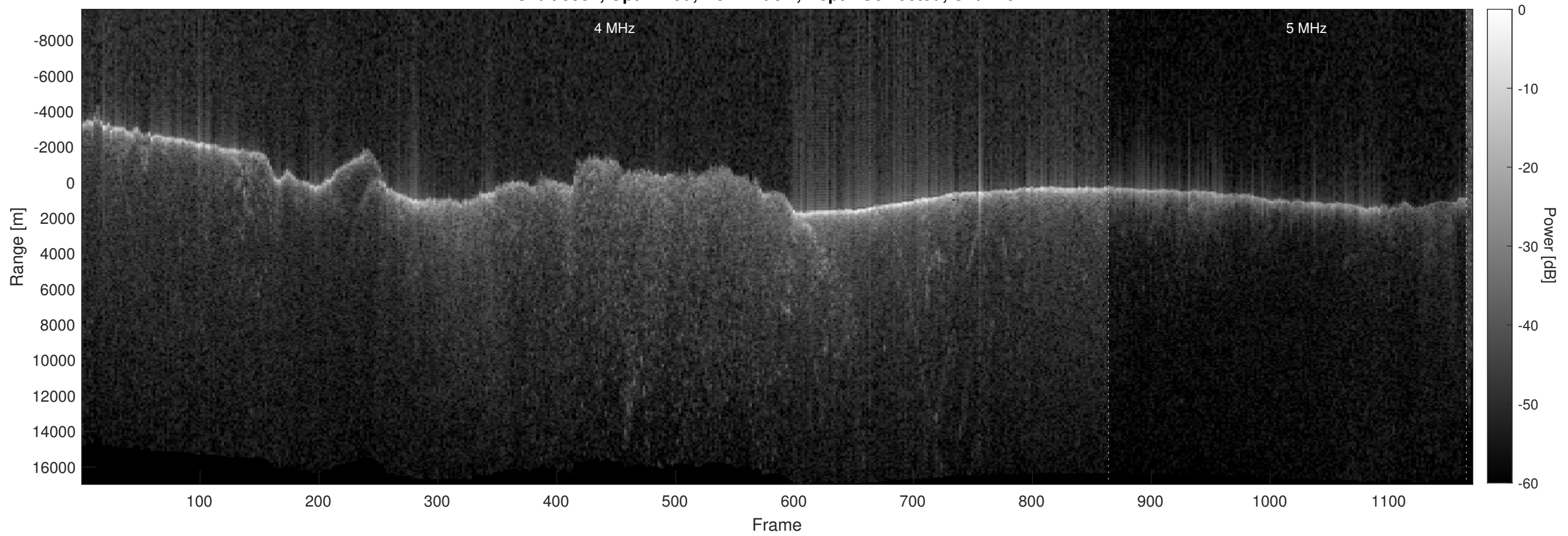
Orbit 5954, Optimized, No Window, Depth-Corrected, Channel 2
