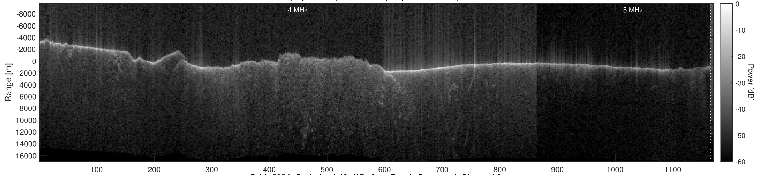
Orbit 5954, Optimized, No Window, Depth-Corrected, Channel 2
