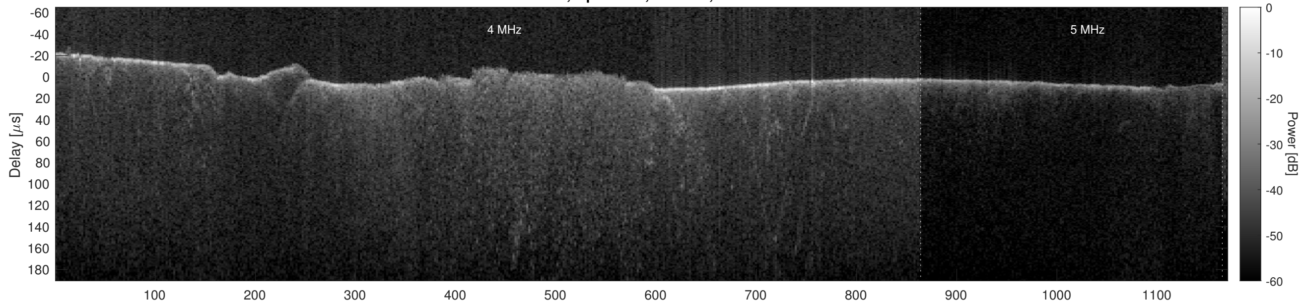
Orbit 5954, Optimized, Window, Channel 2
