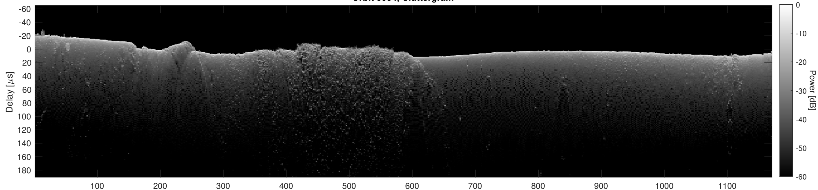
Orbit 5954, Cluttergram
