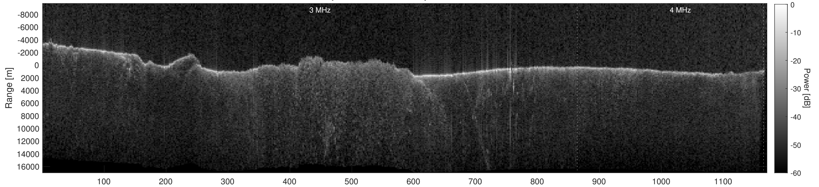
Orbit 5954, Depth-Corrected Cluttergram
