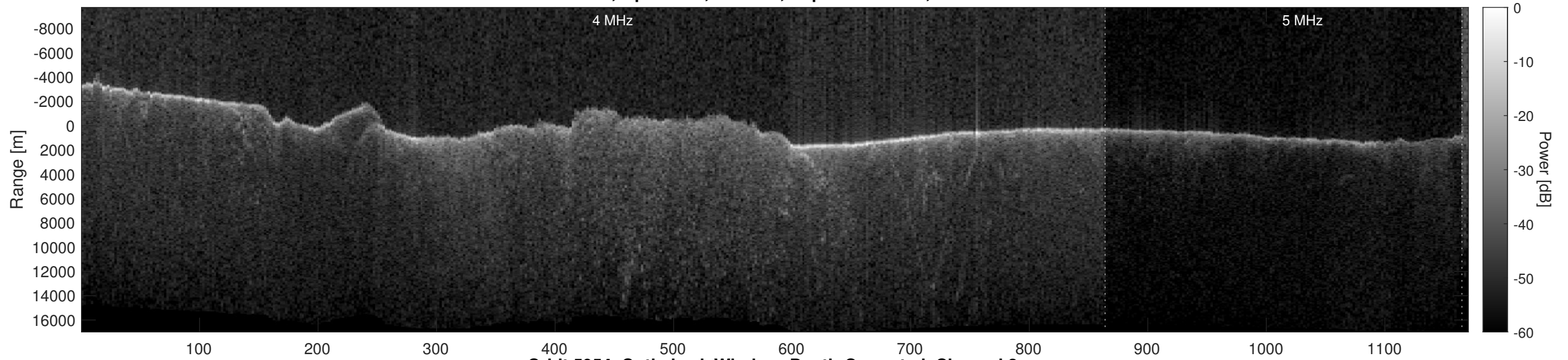
Orbit 5954, Optimized, Window, Depth-Corrected, Channel 2
