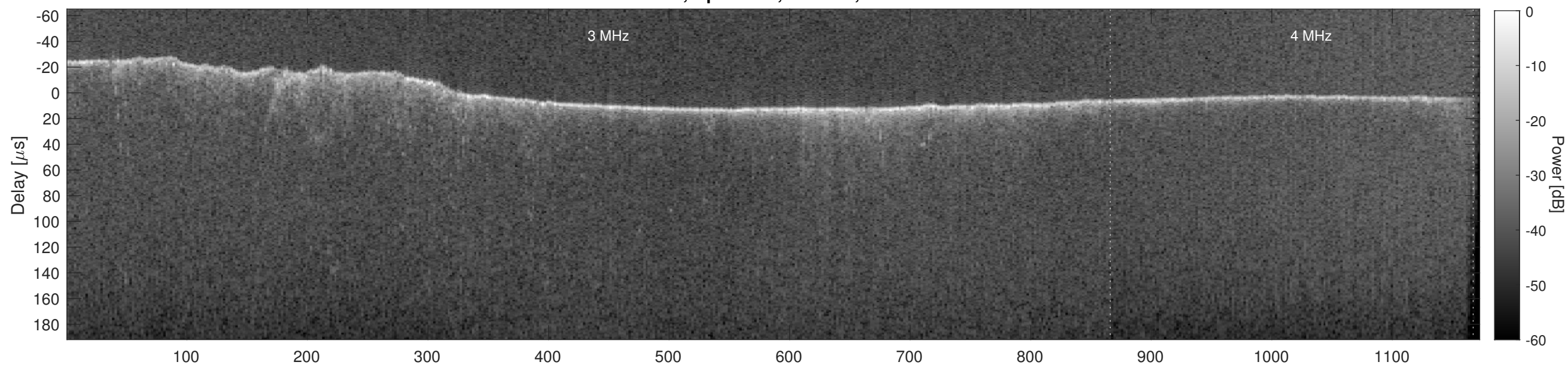
Orbit 5955, Cluttergram
