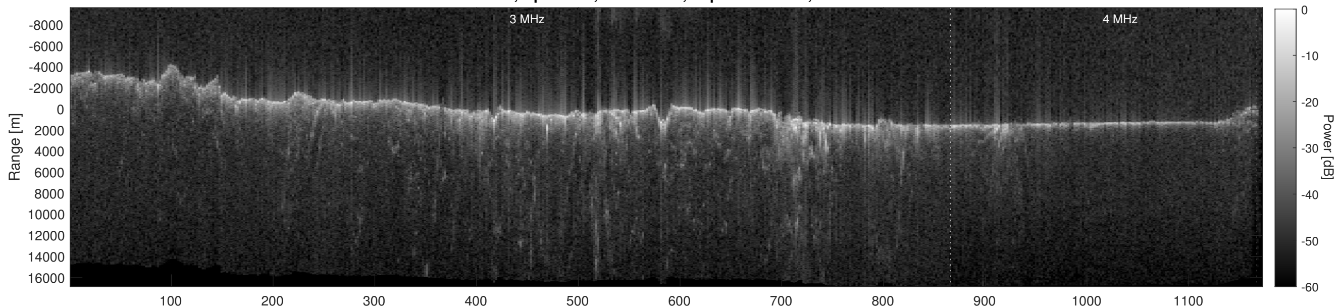
Orbit 5956, Depth-Corrected Cluttergram
