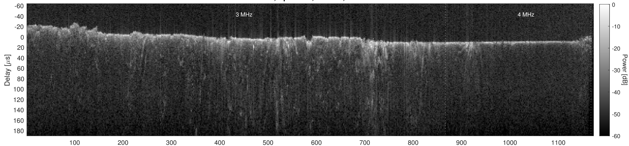
Orbit 5956, Cluttergram
