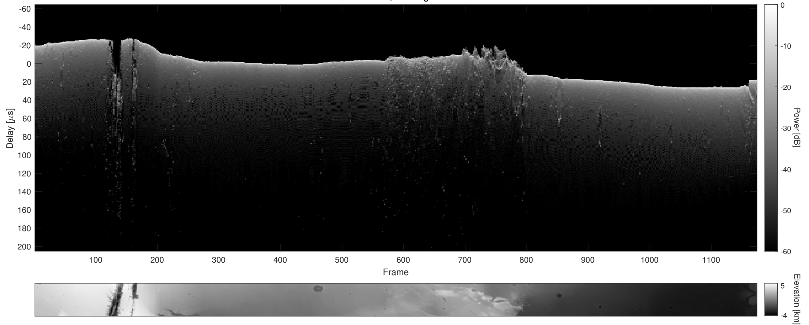
Orbit 5957, Cluttergram
