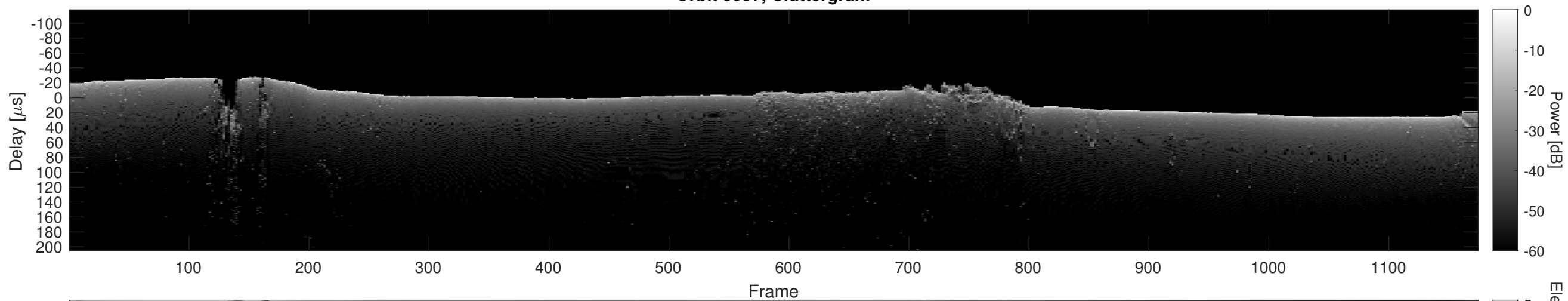
Orbit 5957, Cluttergram
