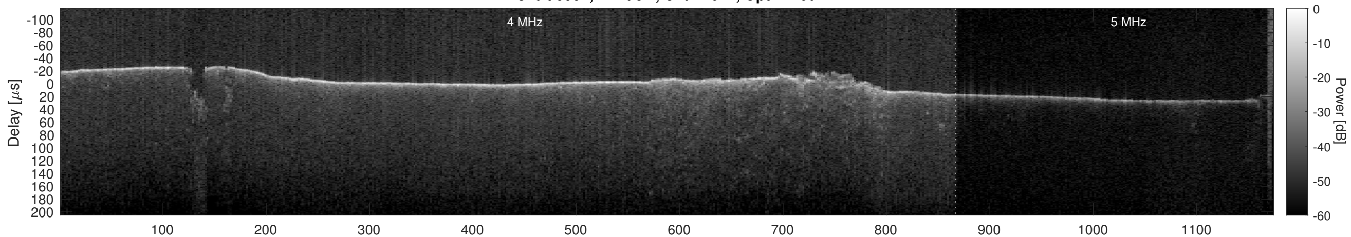
Orbit 5957, Cluttergram
