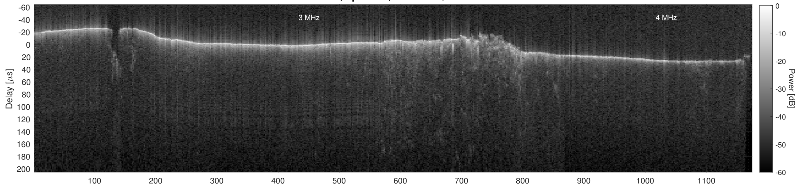
Orbit 5957, Cluttergram
