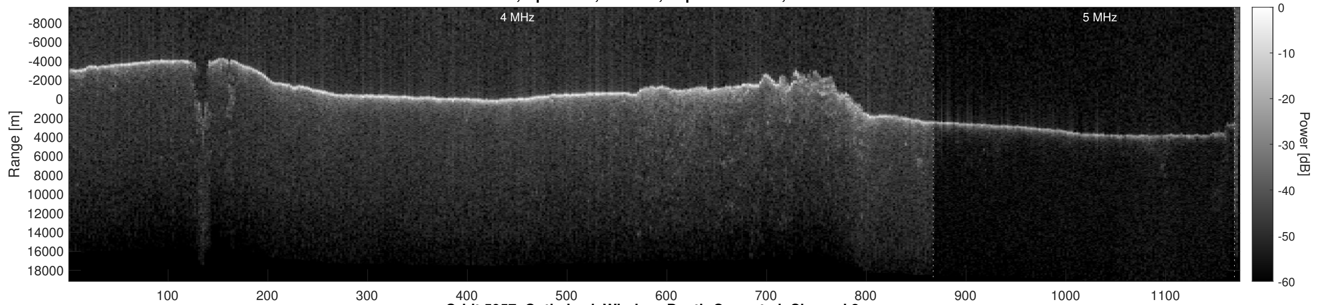
Orbit 5957, Optimized, Window, Depth-Corrected, Channel 2
