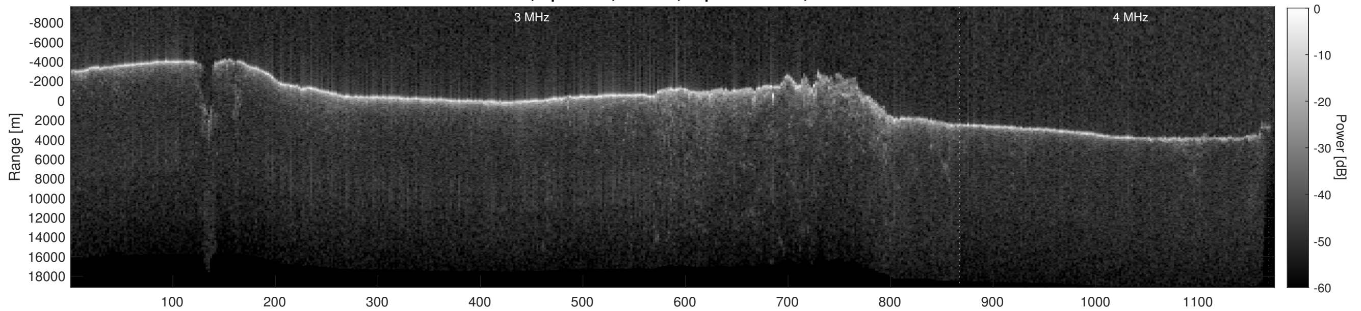
Orbit 5957, Depth-Corrected Cluttergram
