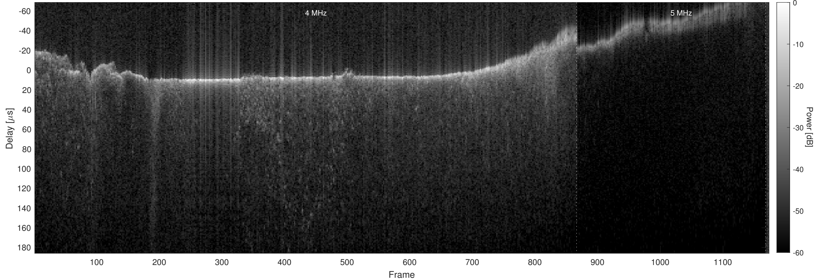
Orbit 5958, Chapman, No Window, Channel 2
