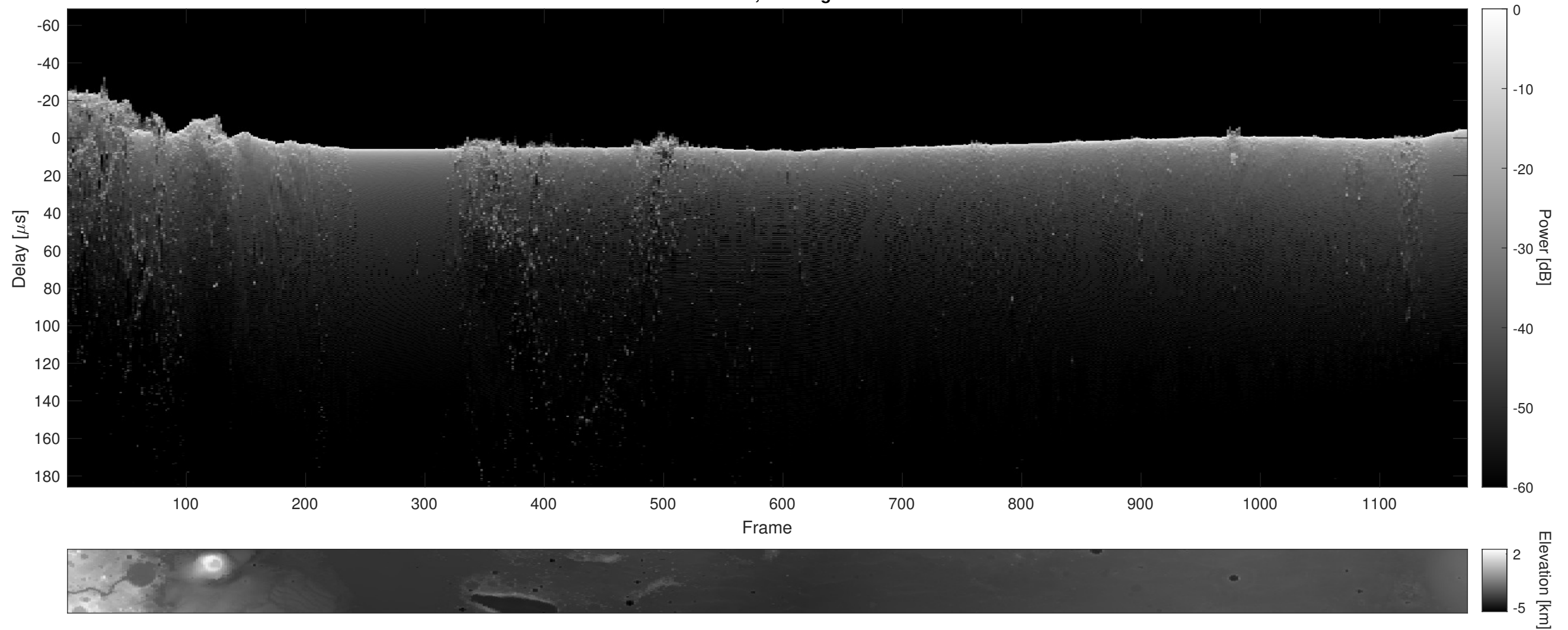
Orbit 5958, Cluttergram
