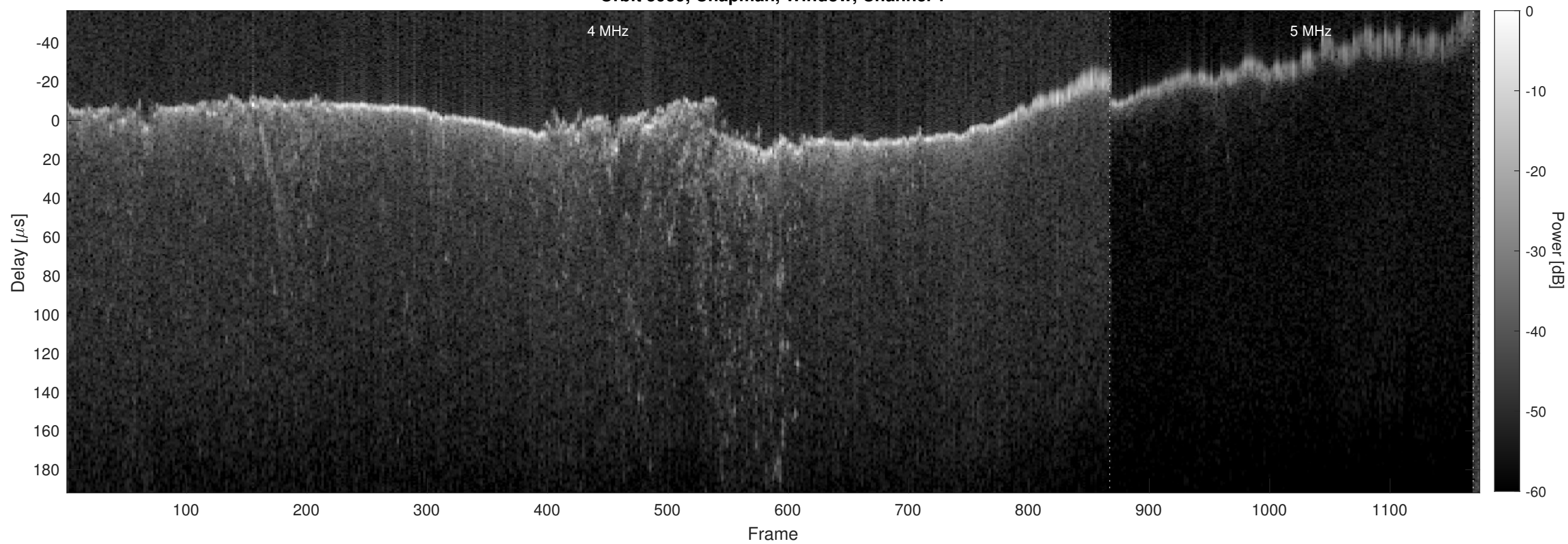
Orbit 5959, Chapman, Window, Channel 2
