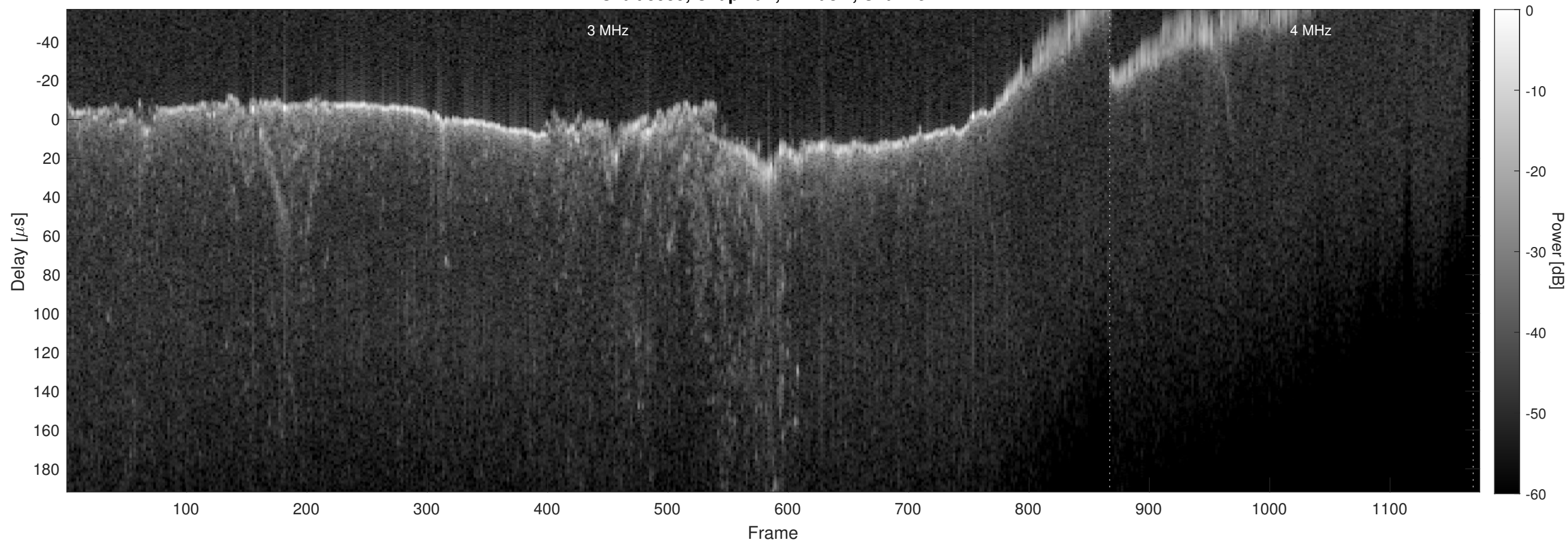
Orbit 5959, Chapman, Window, Channel 2
