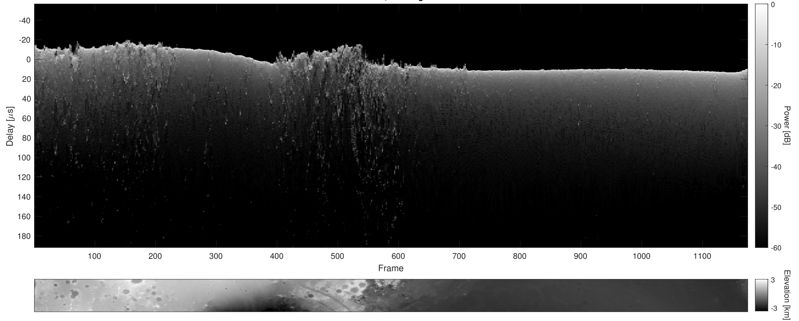
Orbit 5959, Cluttergram
