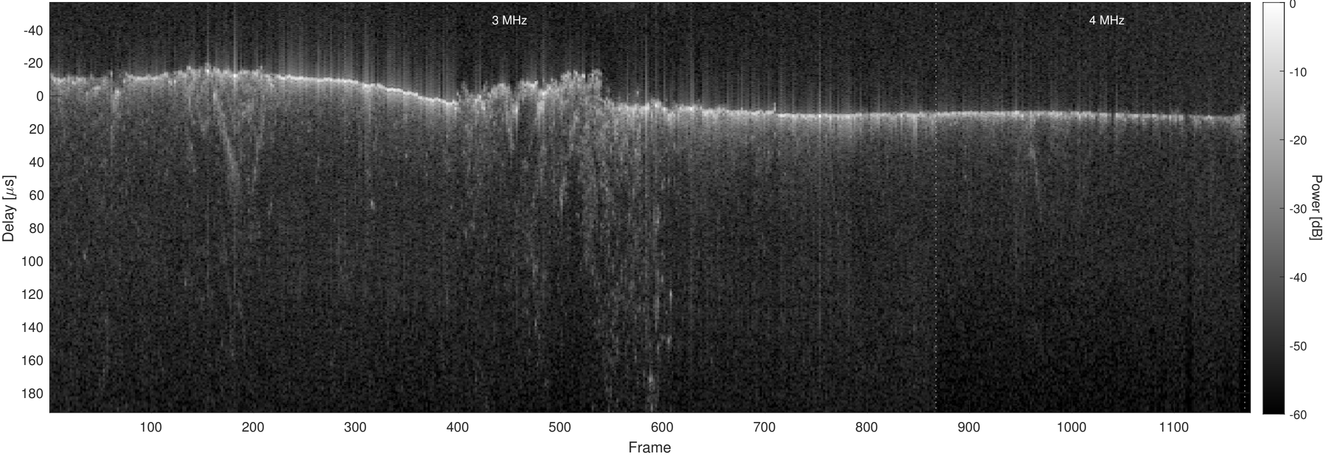
Orbit 5959, Optimized, No Window, Channel 2
